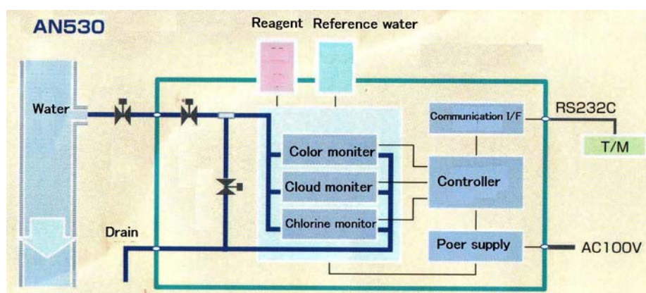
Water-analysis system
