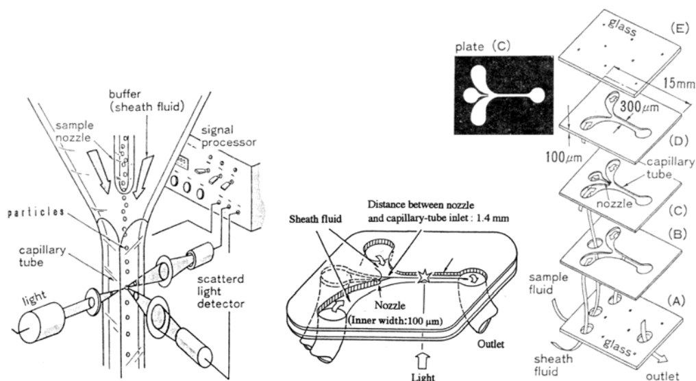
Micro sheath flow chamber for flow cytometer
