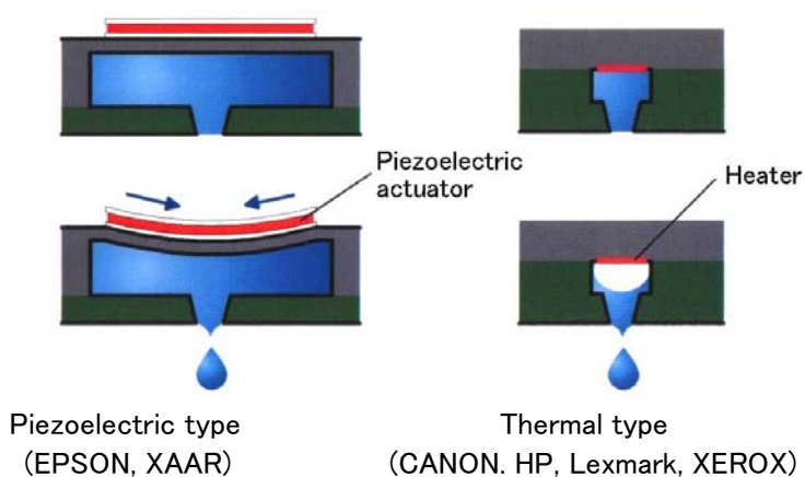
Principle of ink droplet ejection
