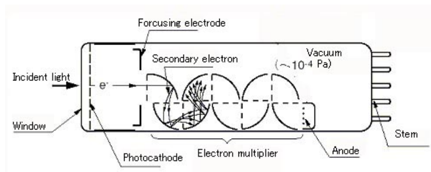
Photomultiplier
