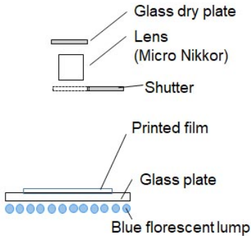
1/20 reduction camera (exhibited)
