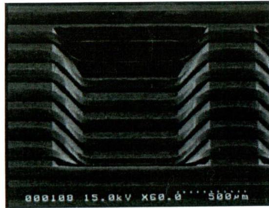
Cross over patterning on 300micro meter trench
