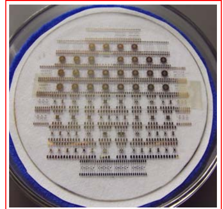
Metal patterning by dry etching
