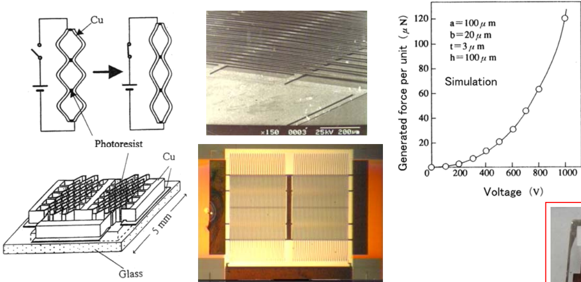
Distributed electrostatic micro actuator
