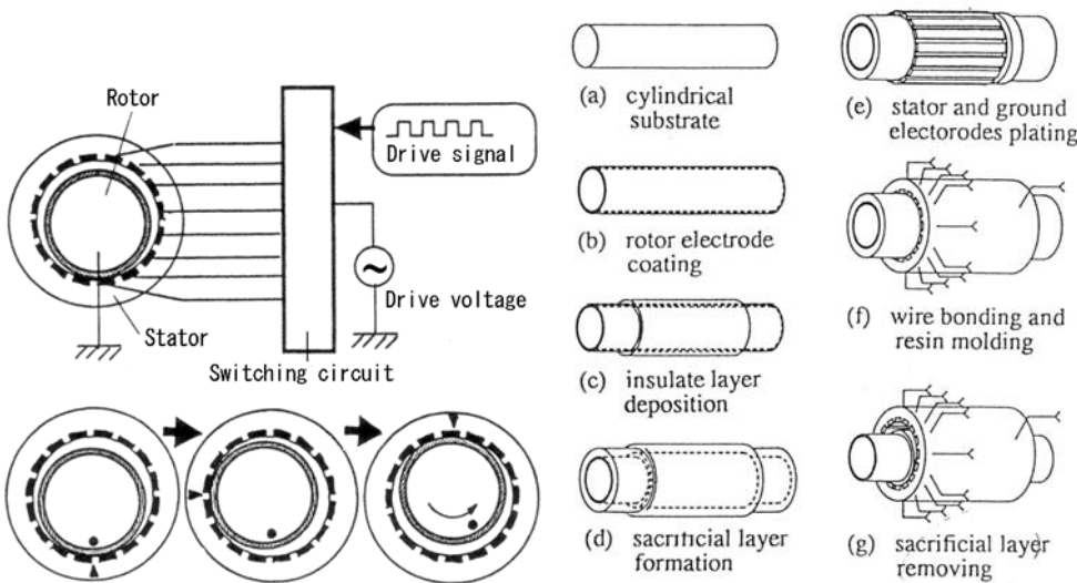
Electrostatic wobble motor (Panasonic Research Institute)
