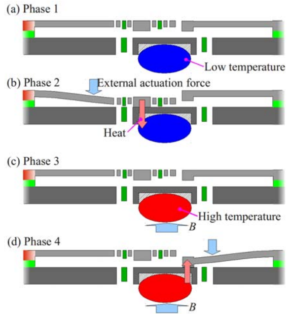
Refrigeration cycle (a)Adiabatic demagnetization (b)Heat dissipation from cold plate (c)Adiabatic magnetization (d)Heat dissipation to ambient.
