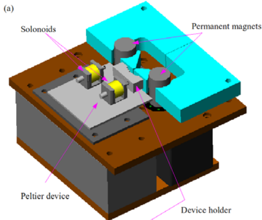
Micro magnetic refrigerator for cooling of micro devices
