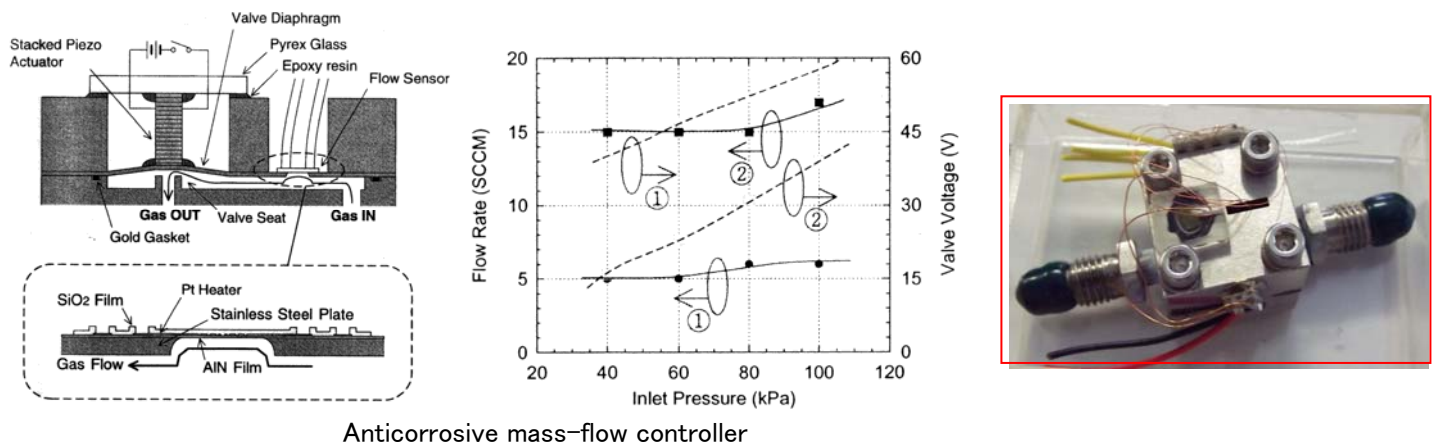
Anticorrosive mass-flow controller
