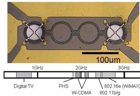
Micro disk resonator (Tohoku Univ. - National Institute of Communication Technology (NICT))
