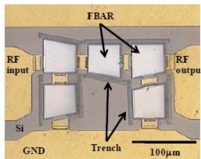
FBAR (Film Bulk Acoustic Resonator) (Tohoku Univ. - National Institute of Communication Technology (NICT))
