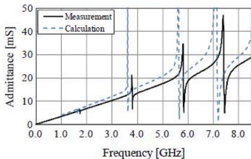
FBAR (Film Bulk Acoustic Resonator) (Tohoku Univ. - National Institute of Communication Technology (NICT))
