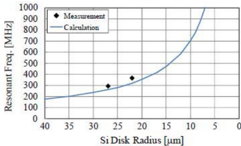
Micro disk resonator (Tohoku Univ. - National Institute of Communication Technology (NICT))
