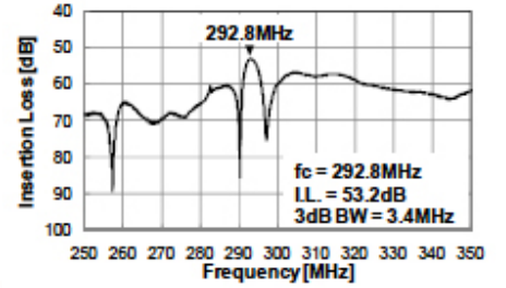
Micro disk resonator (Tohoku Univ. - National Institute of Communication Technology (NICT))
