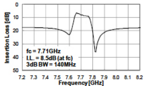
FBAR (Film Bulk Acoustic Resonator) (Tohoku Univ. - National Institute of Communication Technology (NICT))
