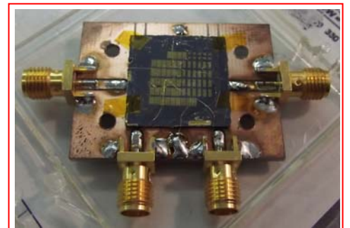
Micro disk resonator (Tohoku Univ. - National Institute of Communication Technology (NICT))
