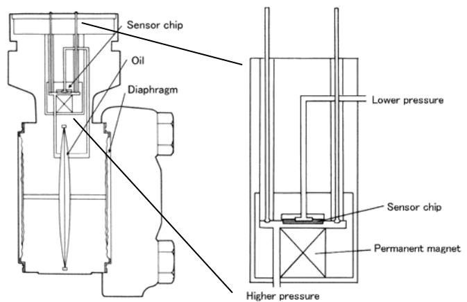
Differential pressure transmitter (DP harp)
