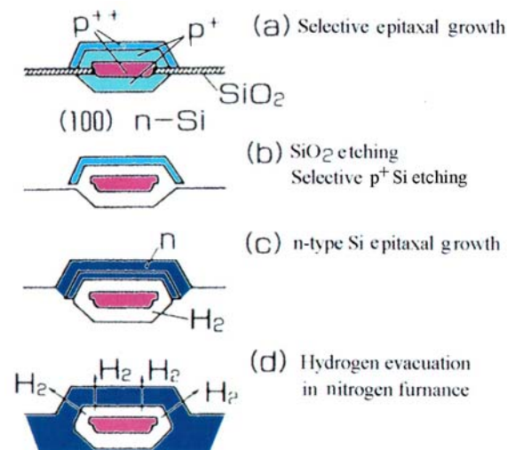
Fabrication process
