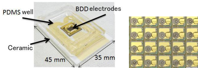
BioLSI made by the transfer of boro doped diamond (BDD) film on LSI (Matsue)
