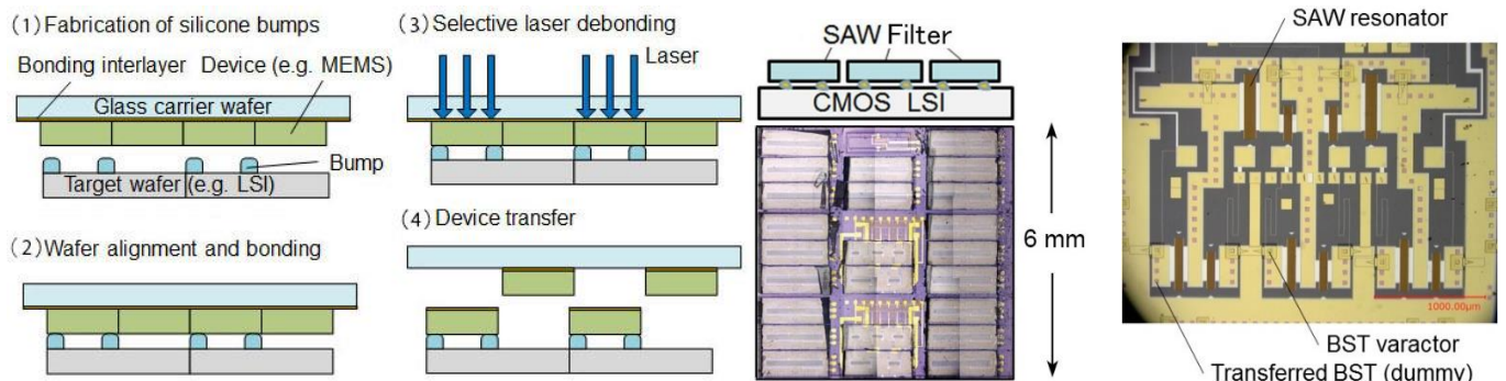
Selective transfer process and multi SAW filter on LSI bade by the process
