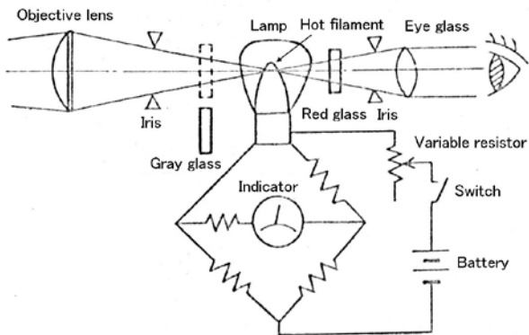
Radiation temperature meter using diminishing image of hot wire
