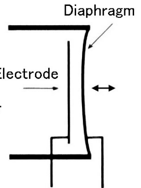
Condenser microphone
