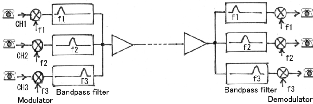
(c) Multiplied communication using unloaded cable (S.Matsumae (1932))
